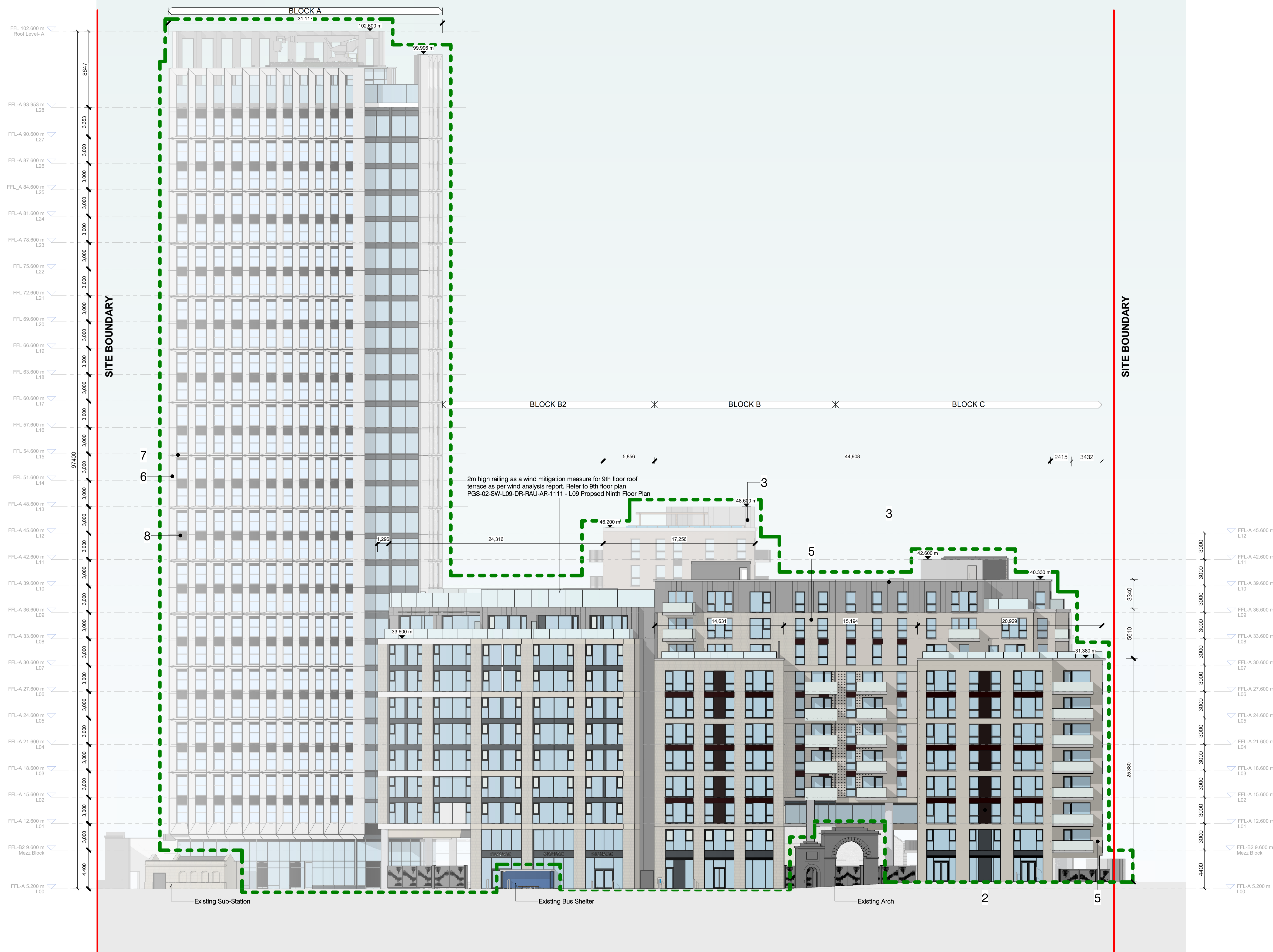
North General Arrangement Elevation 1 : 200
