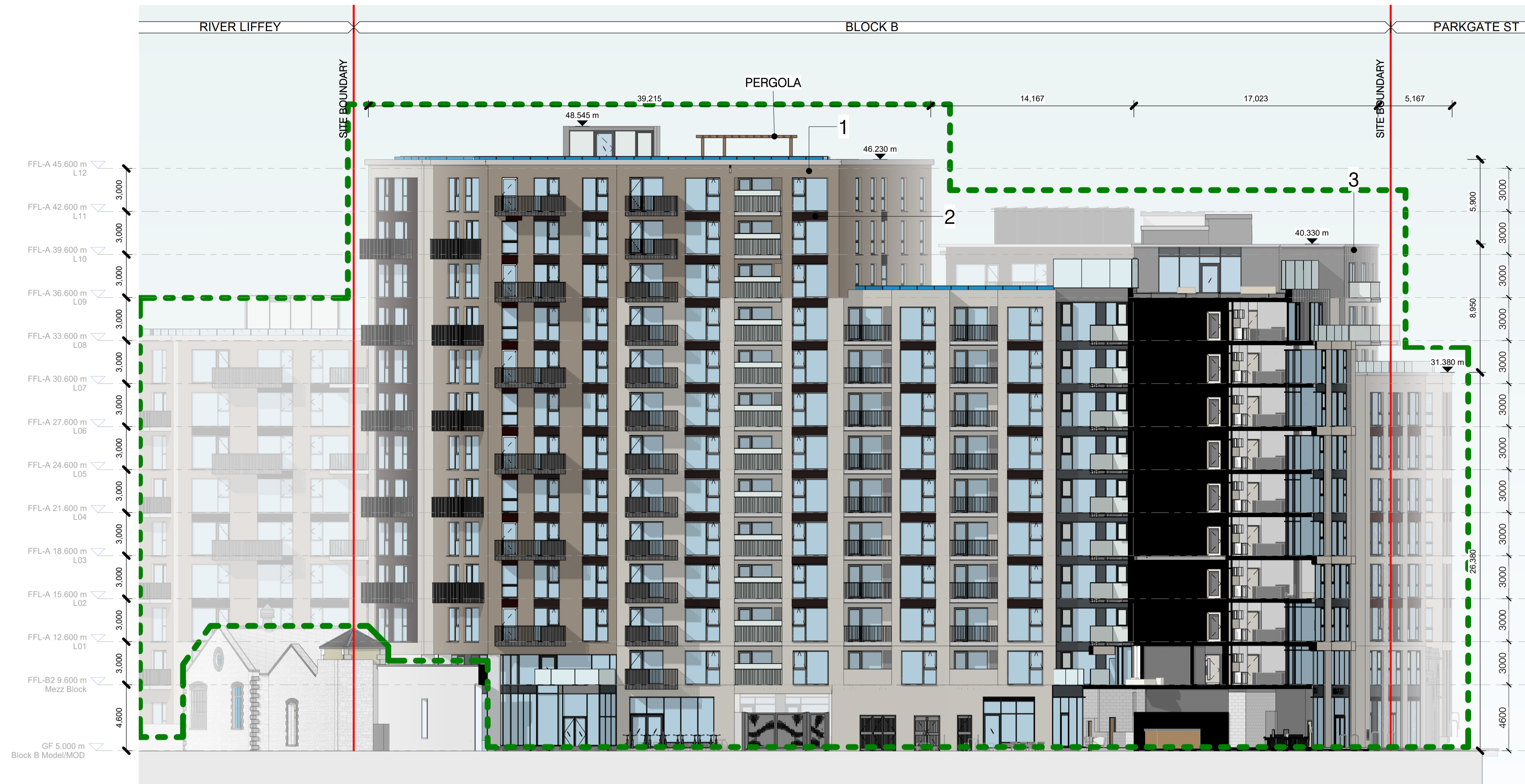
Block B - Proposed East Elevation 1 : 200
