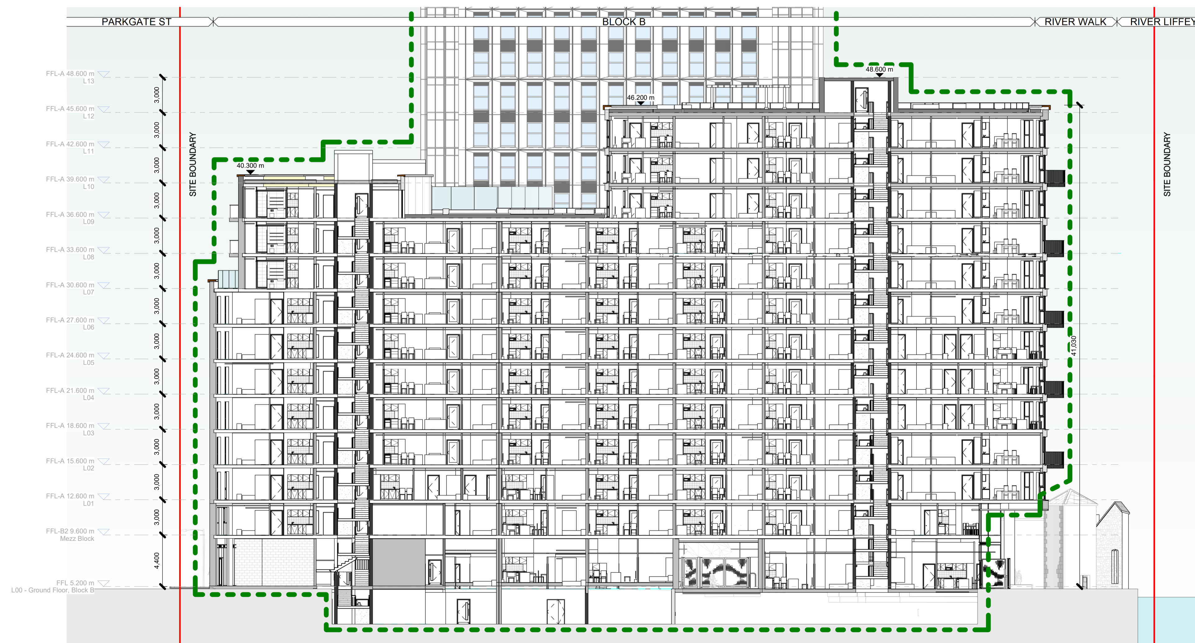
Proposed Section Block B 2-2 1 : 200
