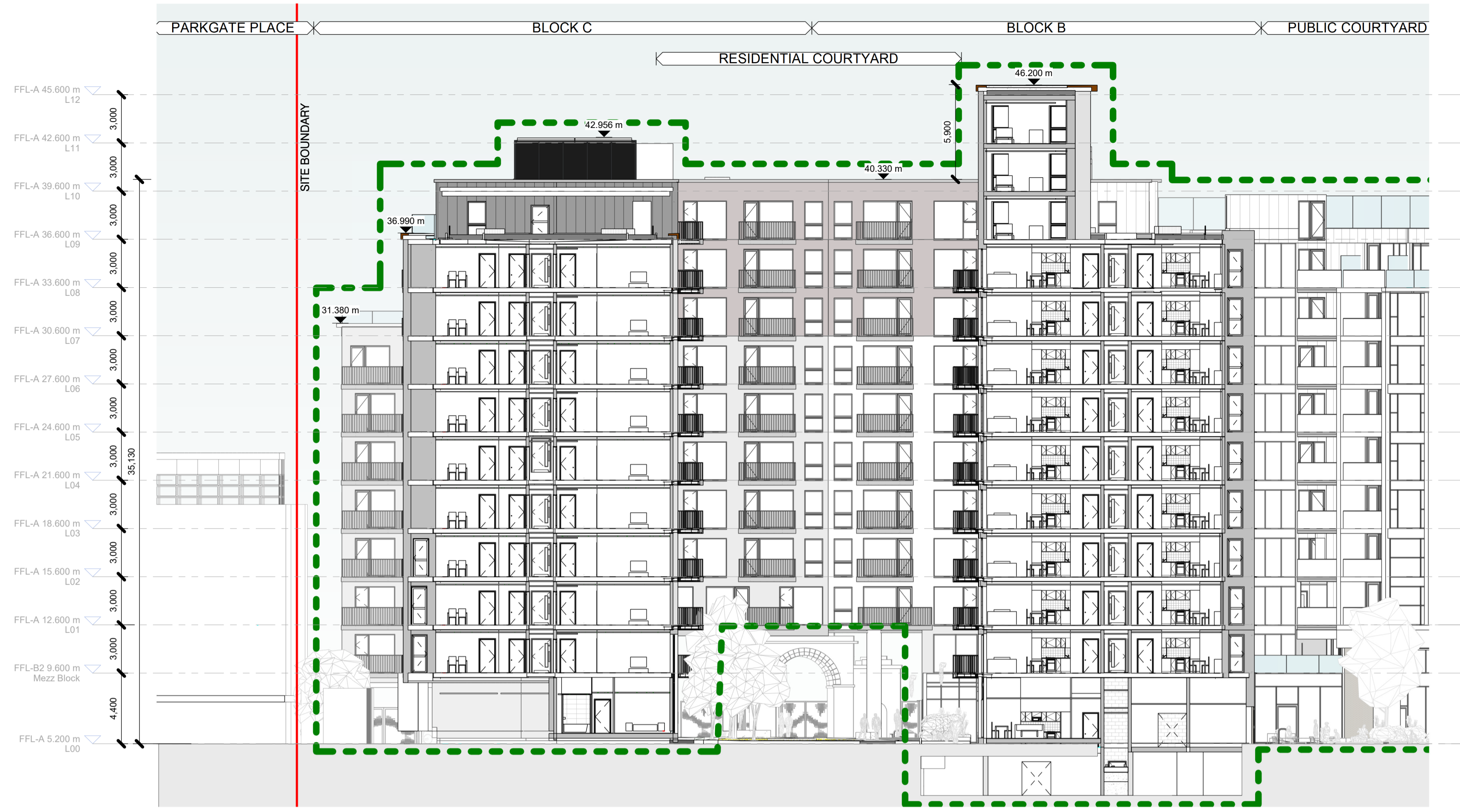
Proposed Section BC 3-3 1 : 200
