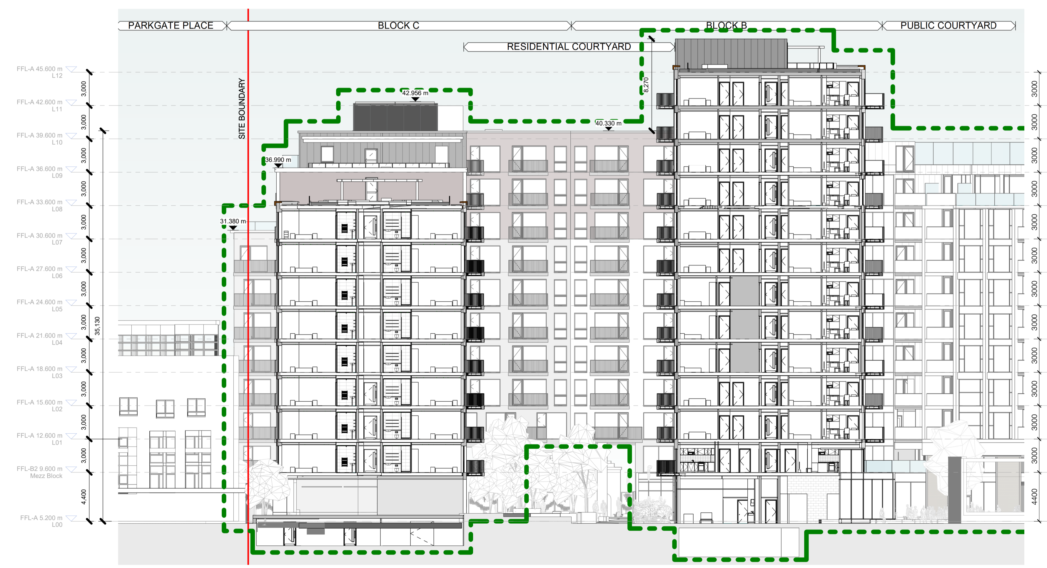
Proposed Section BC 4-4 1 : 200
