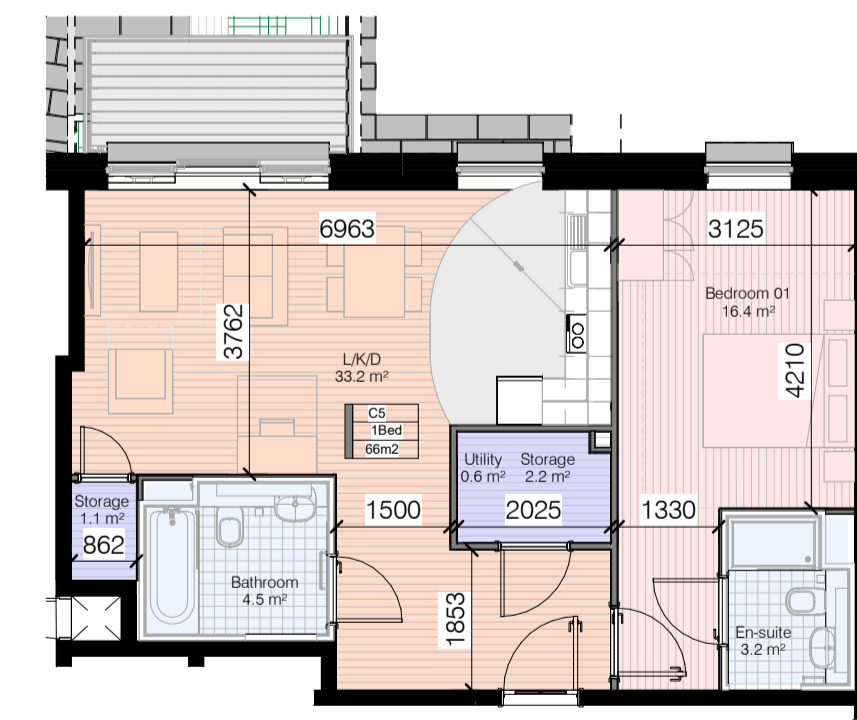
Apt Type 1 Bed (N)-7th-8th Floor-(2P) 1 : 100
