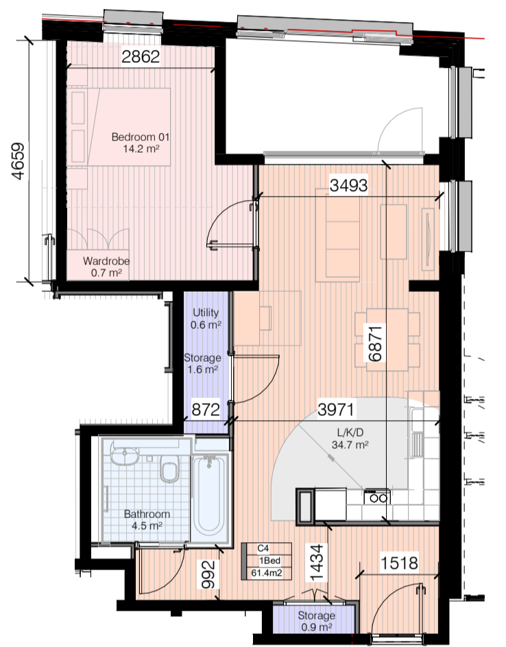
Apt Type 1 Bed (F)-M-1st Floor-(2P) 1 : 100
