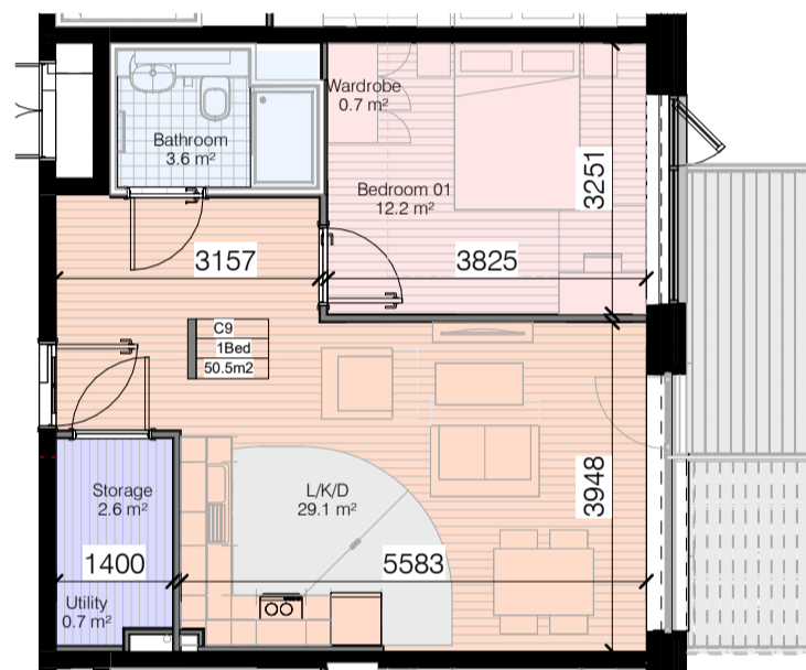
Apt Type 1 Bed (I)-2nd-6th Floor-(2P) 1 : 100
