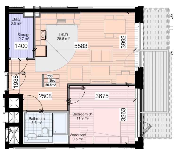
Apt Type 1 Bed (B)-2nd-6th Floor-(2P) 1 : 100
