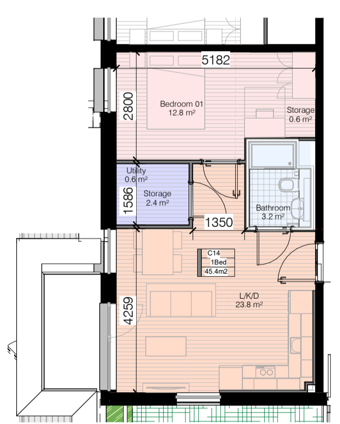
Apt Type 1 Bed (M)-9th Floor-(2P) 1 : 100
