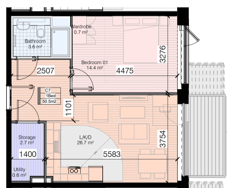
Apt Type 1 Bed (G)-2nd-6th Floor-(2P) 1 : 100
