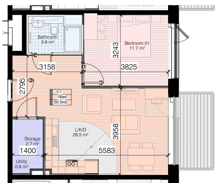
Apt Type 1 Bed (A)-2nd-6th Floor-(2P) 1 : 100
