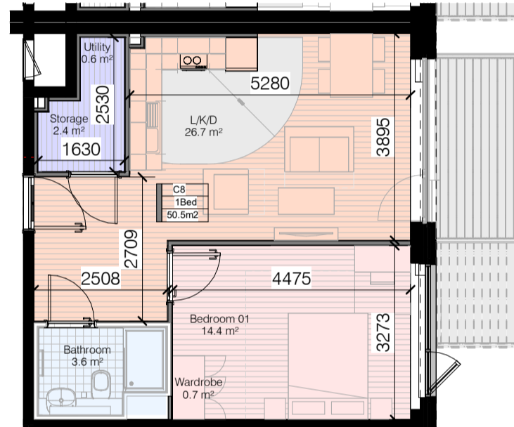
Apt Type 1 Bed (H)-M-6th Floor-(2P) 1 : 100
