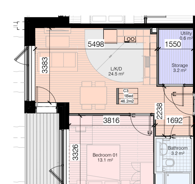
Apt Type 1 Bed (E)-2nd-6th Floor-(2P) 1 : 100
