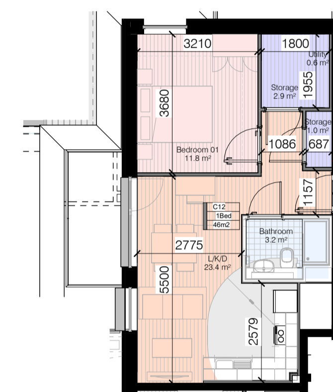
Apt Type 1 Bed (J)-9th Floor-(2P) 1 : 100
