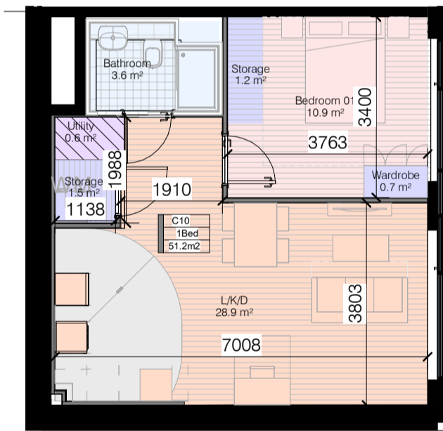
Apt Type 1 Bed (Q)-Ground Floor-(2P) 1 : 100
