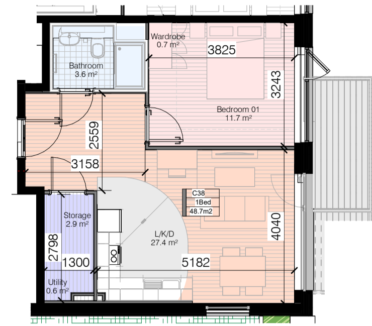
Apt Type 1 Bed (O)-9th Floor-(2P) 1 : 100
