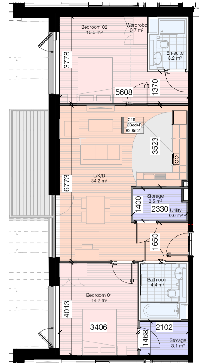
Apt Type 2 Bed (A)-2nd-6th Floor-(4P) 1 : 100
