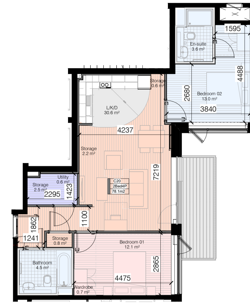
Apt Type 2 Bed (B)-2nd-9th Floor-(4P) 1 : 100
