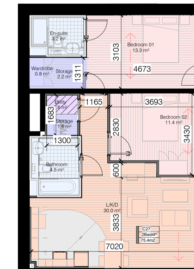
Apt Type 2 Bed (H)-Ground Floor-(4P) 1 : 100
