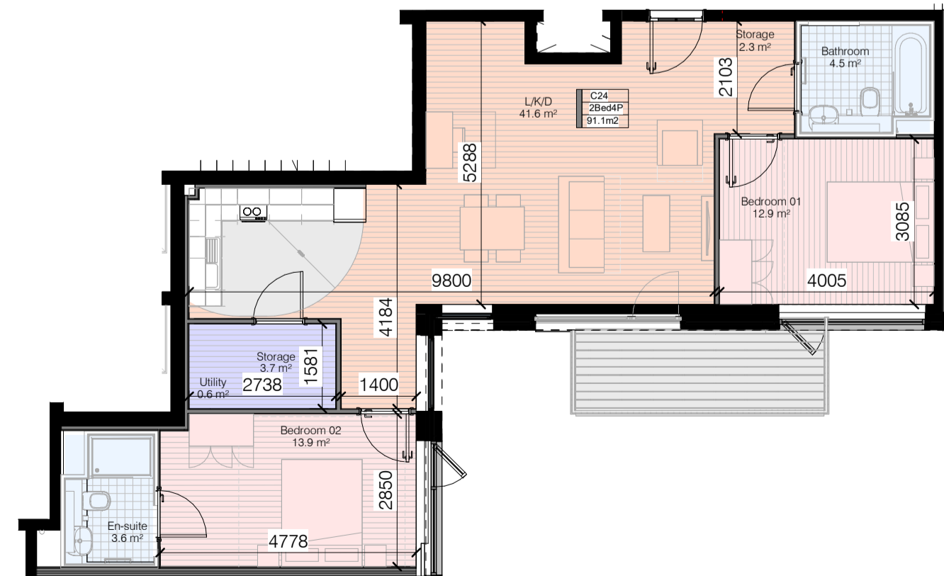
Apt Type 2 Bed (C)-1st Floor-(4P) 1 : 100
