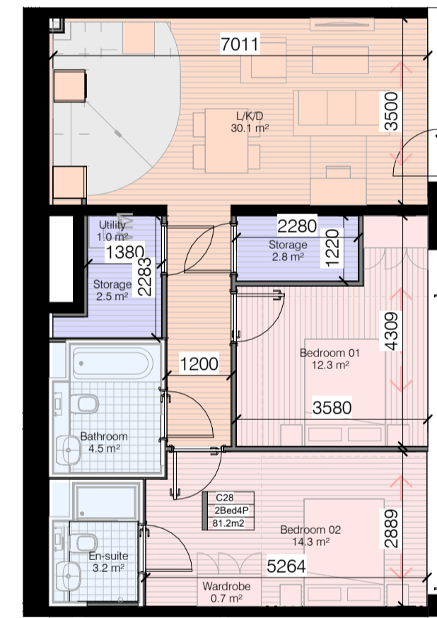
Apt Type 2 Bed (I)-Ground Floor-(4P) 1 : 100
