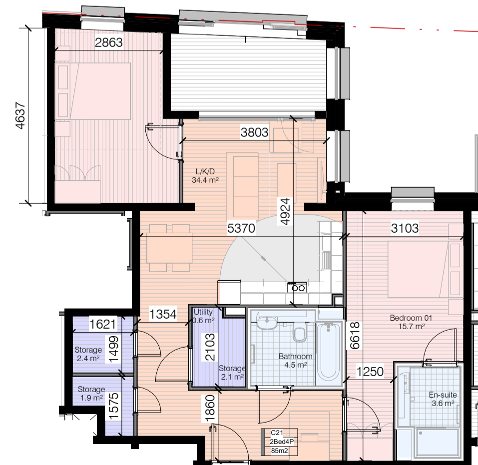
Apt Type 2 Bed (E)-2nd-6th Floor-(4P) 1 : 100
