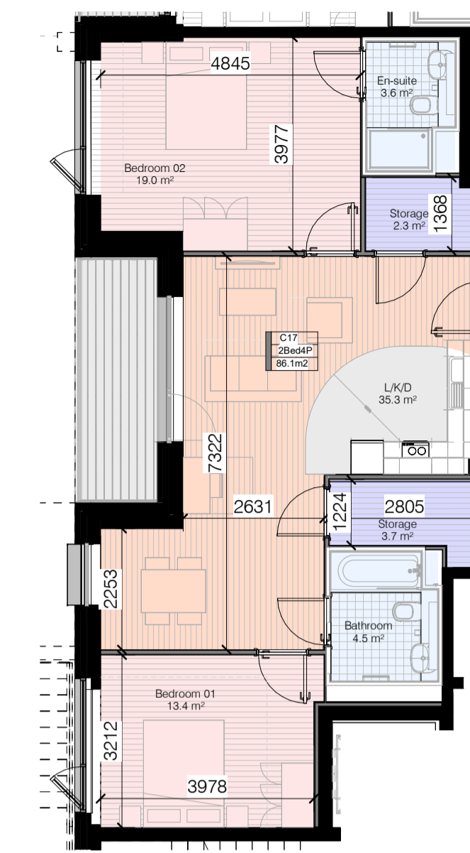
Apt Type 2 Bed (F)-2nd-6th Floor-(4P) 1 : 100
