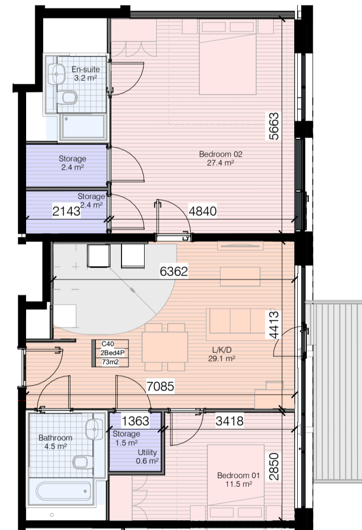
Apt Type 2 Bed (N)-M Floor-(4P) 1 : 100
