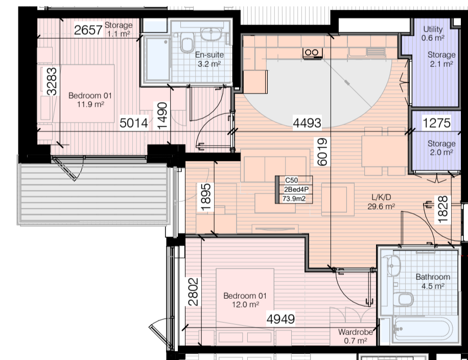
Apt Type 2 Bed (M)-M-6th Floor-(4P) 1 : 100
