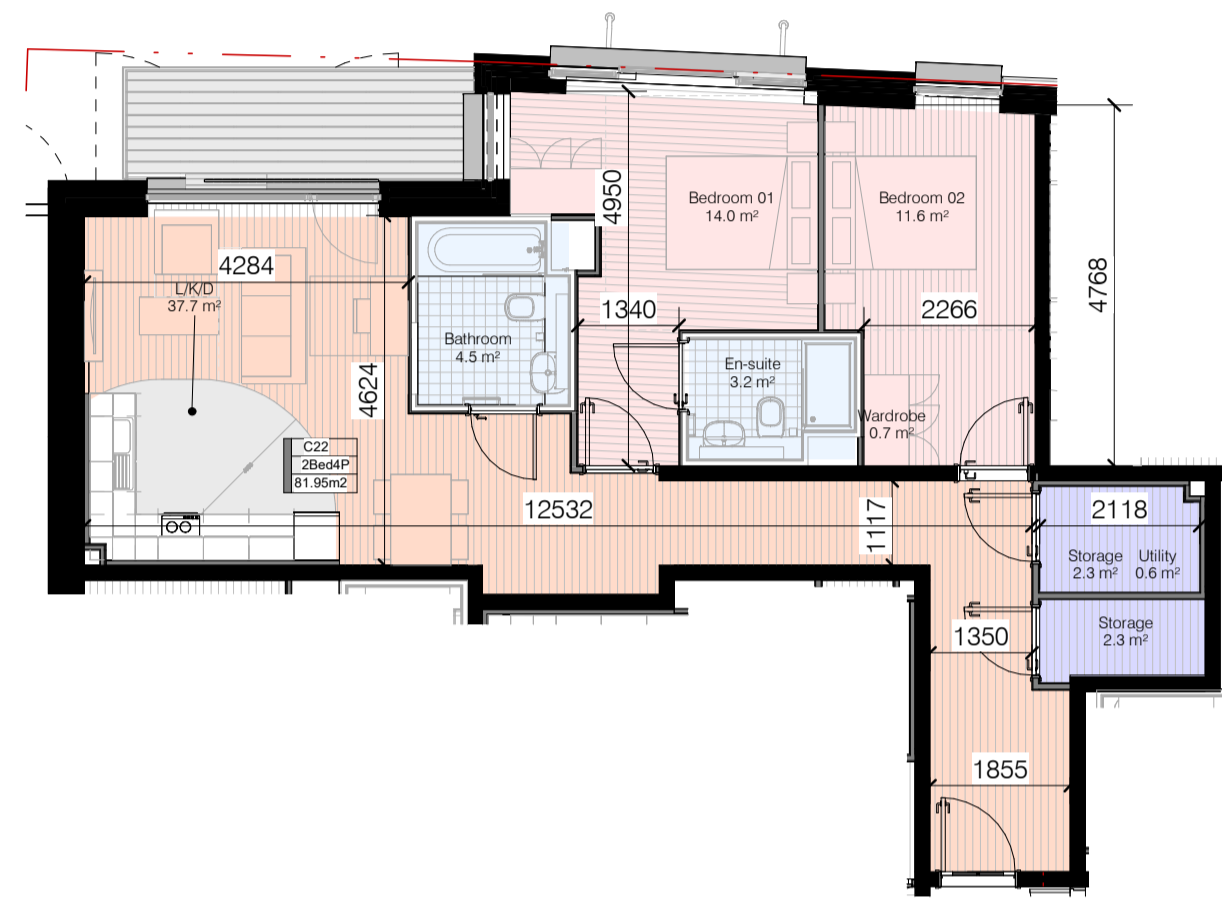
Apt Type 2 Bed (K)-M-6th Floor-(4P) 1 : 100
