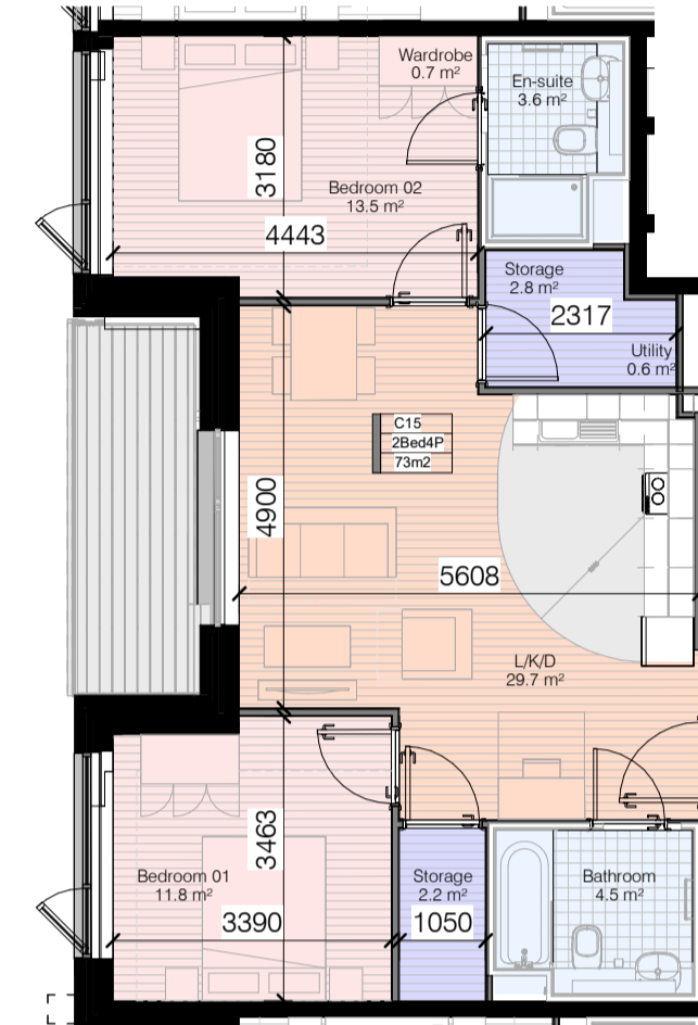
Apt Type 2 Bed (L)-M-8th Floor-(4P) 1 : 100
